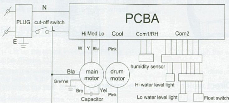
Wiring diagram
